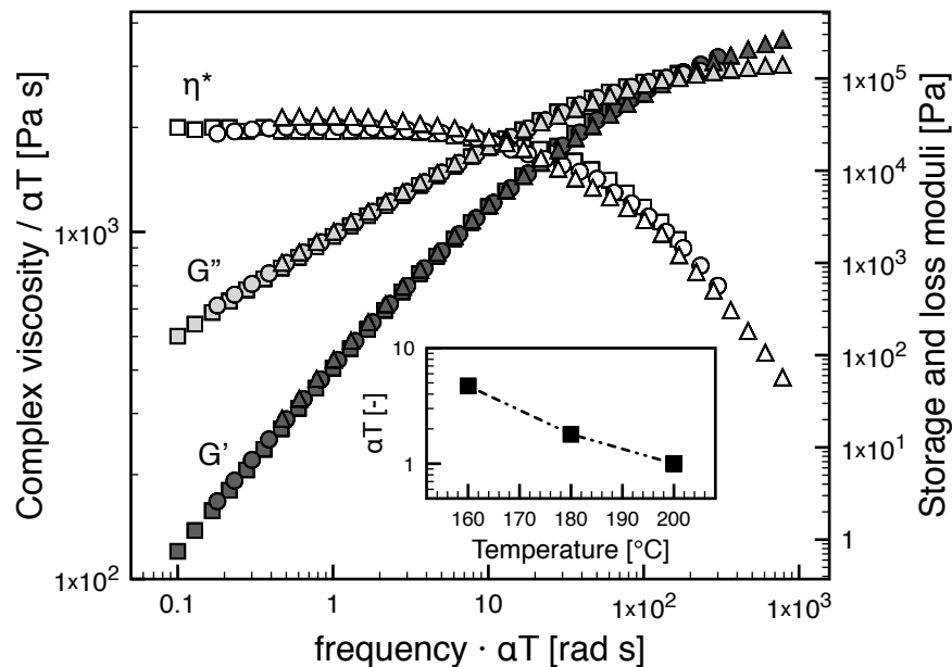
Figure 1. Rheological measurements on PLA Natureworks 4032D.
