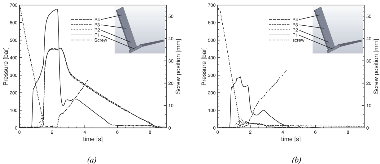
Figure 5. Pressure evolution measured during the injection molding test carried out: a) without gas; b) with gas and a back pressure of 5 bar
