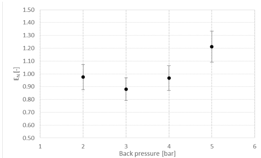
Figure 13 Normalized modulus of elasticity obtained from tensile tests at different back pressures.
