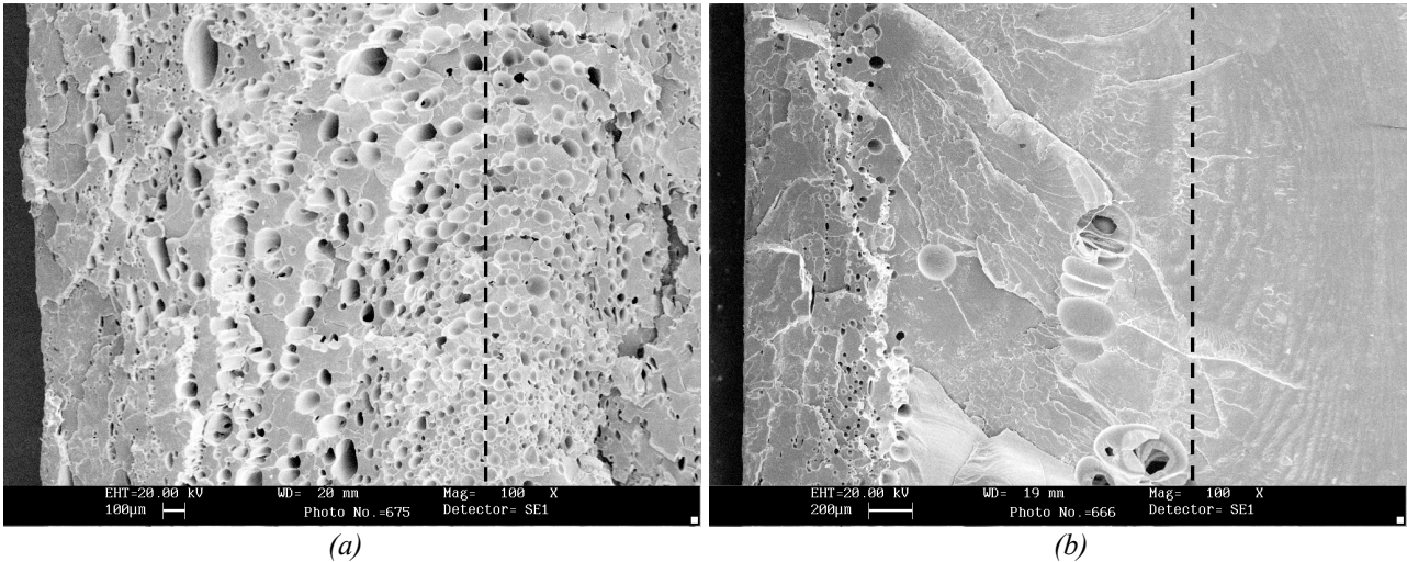
Figure 9. SEM micrographs of the section at 60 mm from the gate (flow/expansion direction toward the reader) of samples molded with back pressure 3 bar and 5 bar respectively. The midplane is marked with dotted lines.
