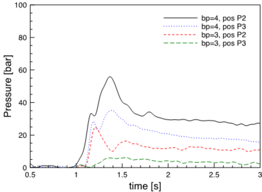
Figure 11. Pressure profiles measured for two different back pressures.
