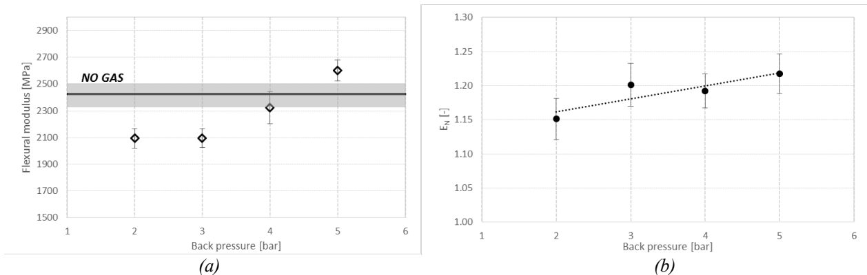
Figure 12. (a) Modules of elasticity obtained by flexural tests at 5 mm/min for PLA 4032D samples foamed with different back pressure; line represents the average value of the flexural modulus of samples without gas; (b) Normalized modulus of elasticity.
